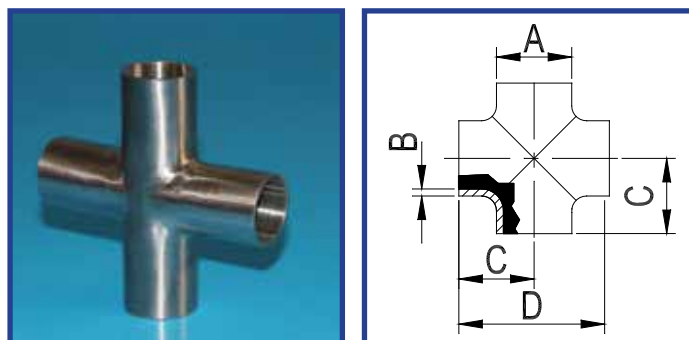
9W (3A) PULLED CROSS 304,304L,316,316L
