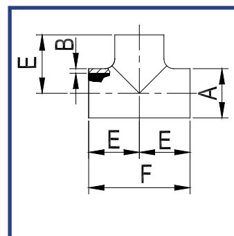
L7WWW (3A) SHORT EQUAL TEE 304,304L,316,316L
