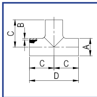
7W (3A) LONG EQUAL TEE 304,304L,316,316L
